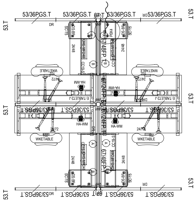
2D PLAN LAYOUT
